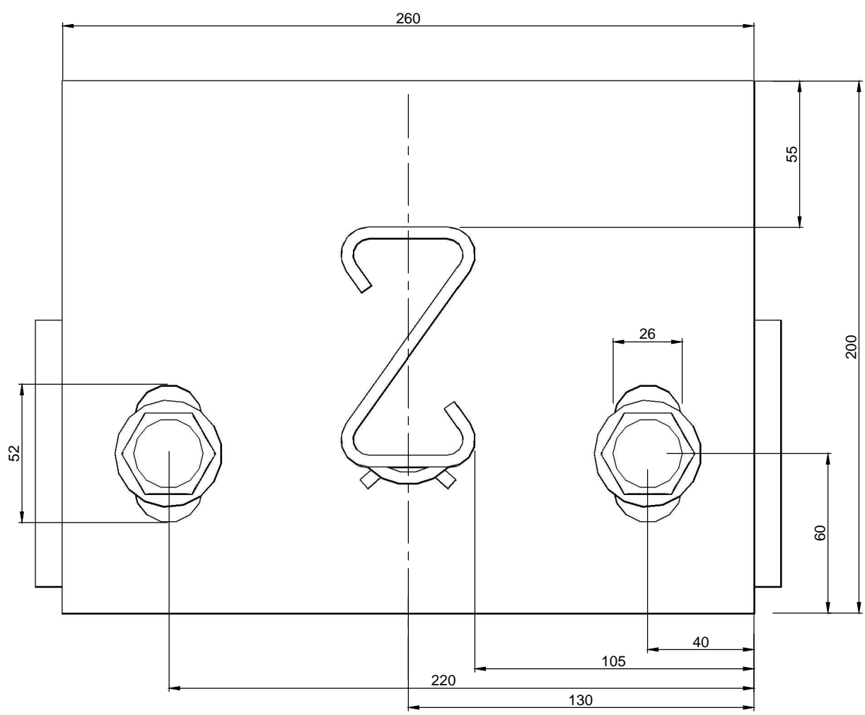
VIEW A
