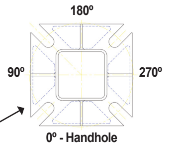
Top View of 5x5 Anchor Base
