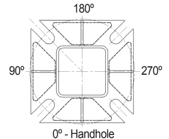
Top View of 5 x 5 Anchor Base
