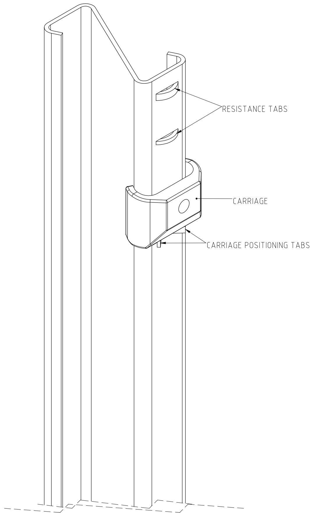
HC "Z" POST & CARRIAGE ASSEMBLY ISOMETRIC VIEW
