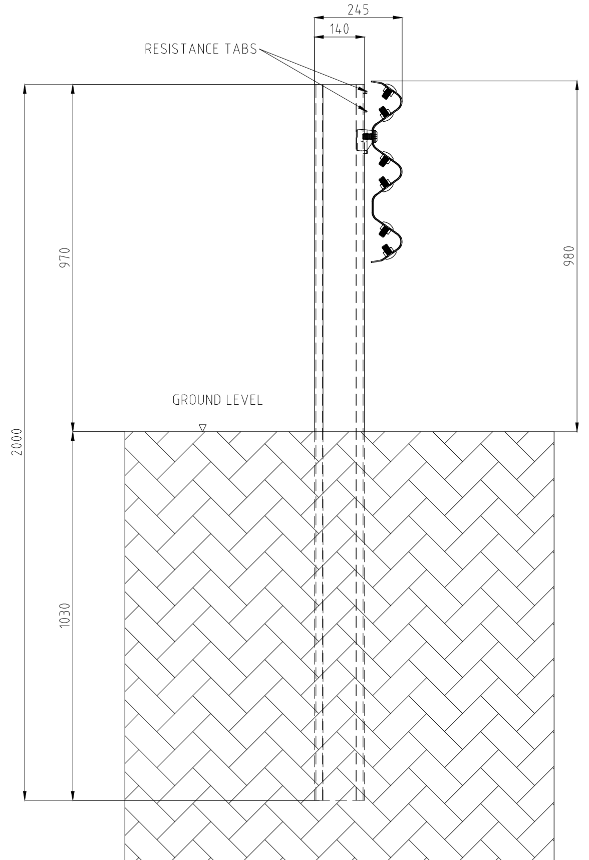
HC "Z" POST & CARRIAGE ASSEMBLY SIDE VIEW
