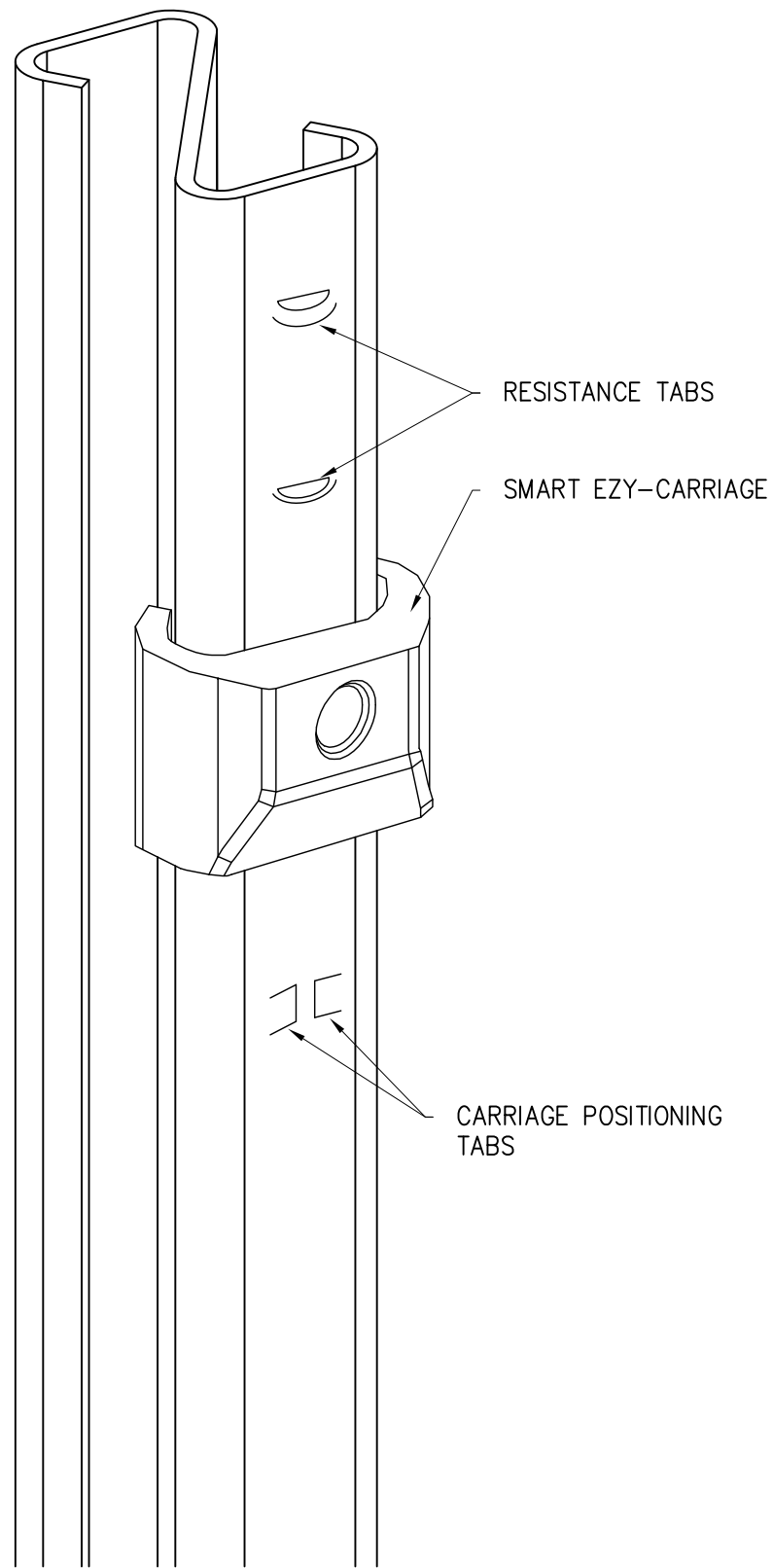
Z-POST & CARRIAGE ASSEMBLY ISOMETRIC VIEW
