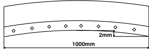
LONGITUDINAL BOW OF LOUVRE BLADE OR FLAT BAR
