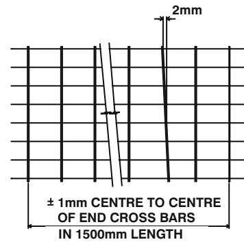
CROSS BAR ALIGNMENT & STRAIGHTNESS
