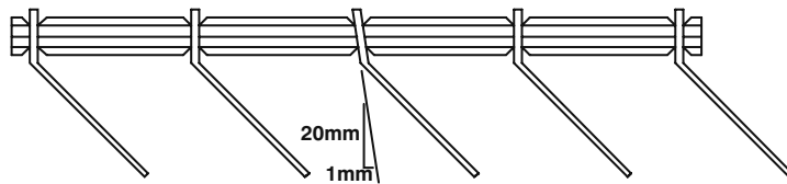
LOUVRE BLADE LEAN
