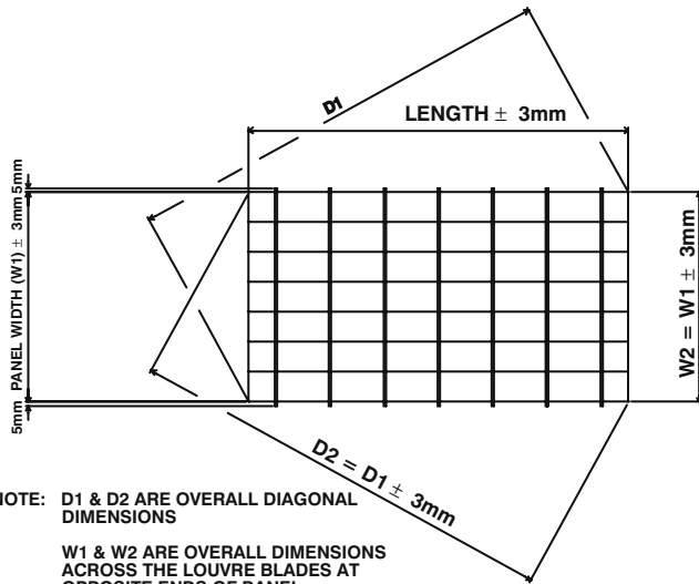
OVERALL DIMENSIONS & SQUARENESS
