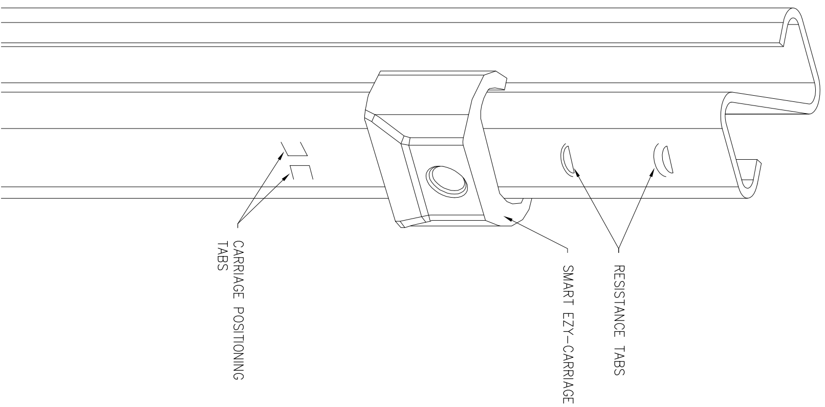
Z-POST & CARRIAGE ASSEMBLY ISOMETRIC VIEW
