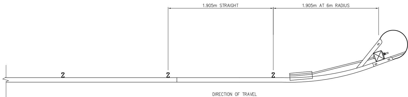
PLAN - CURVED TRAILING TERMINAL 10006725
