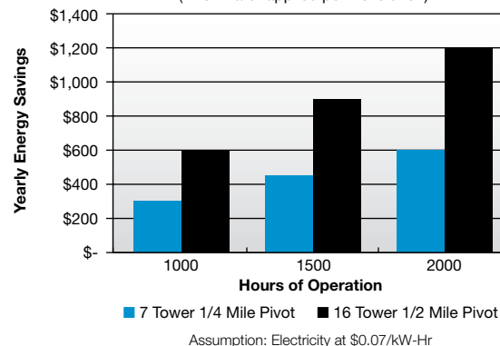
Yearly Energy Savings to run Electric vs. Oil Hydraulic Center Pivot (1" of Water applied per Revolution)
