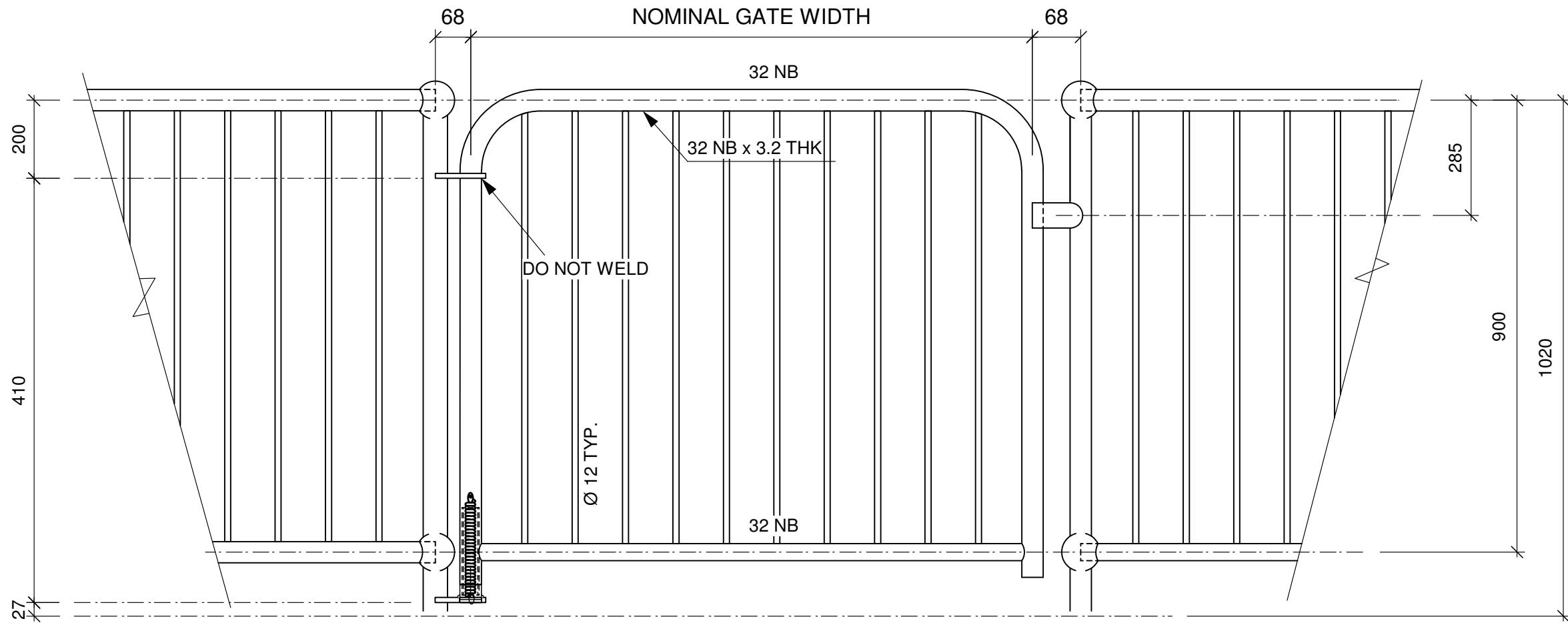
ELEVATION- FENCE (BALUSTRADE) GATE
