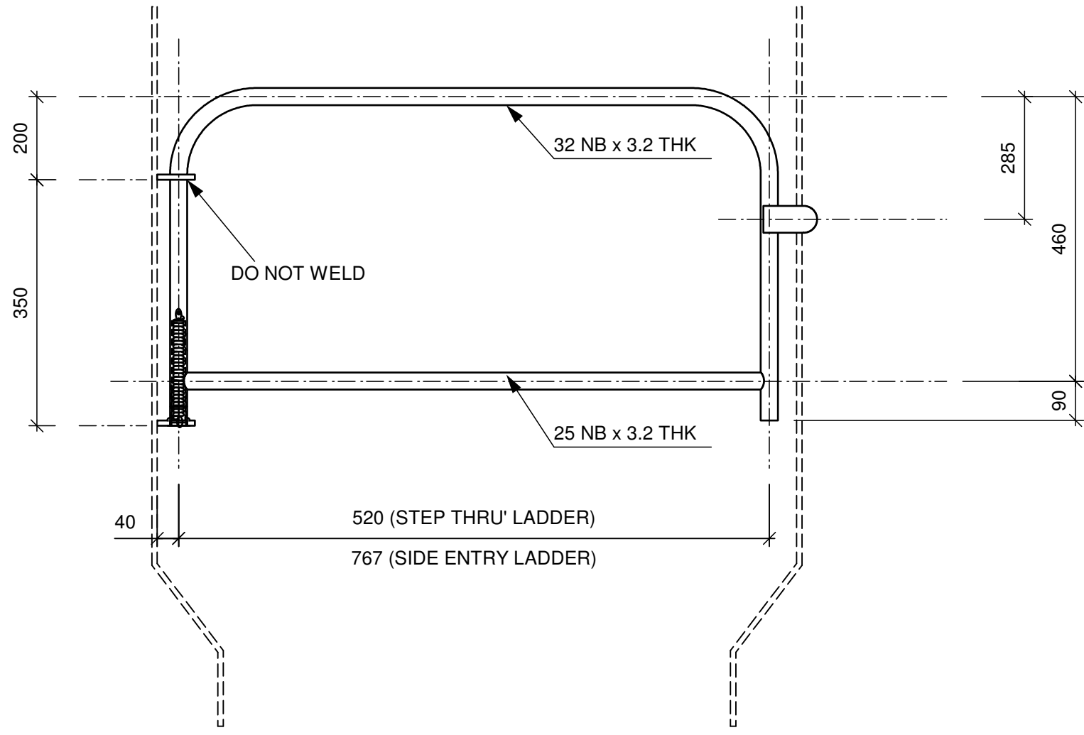
ELEVATION - SELF CLOSING GATE
