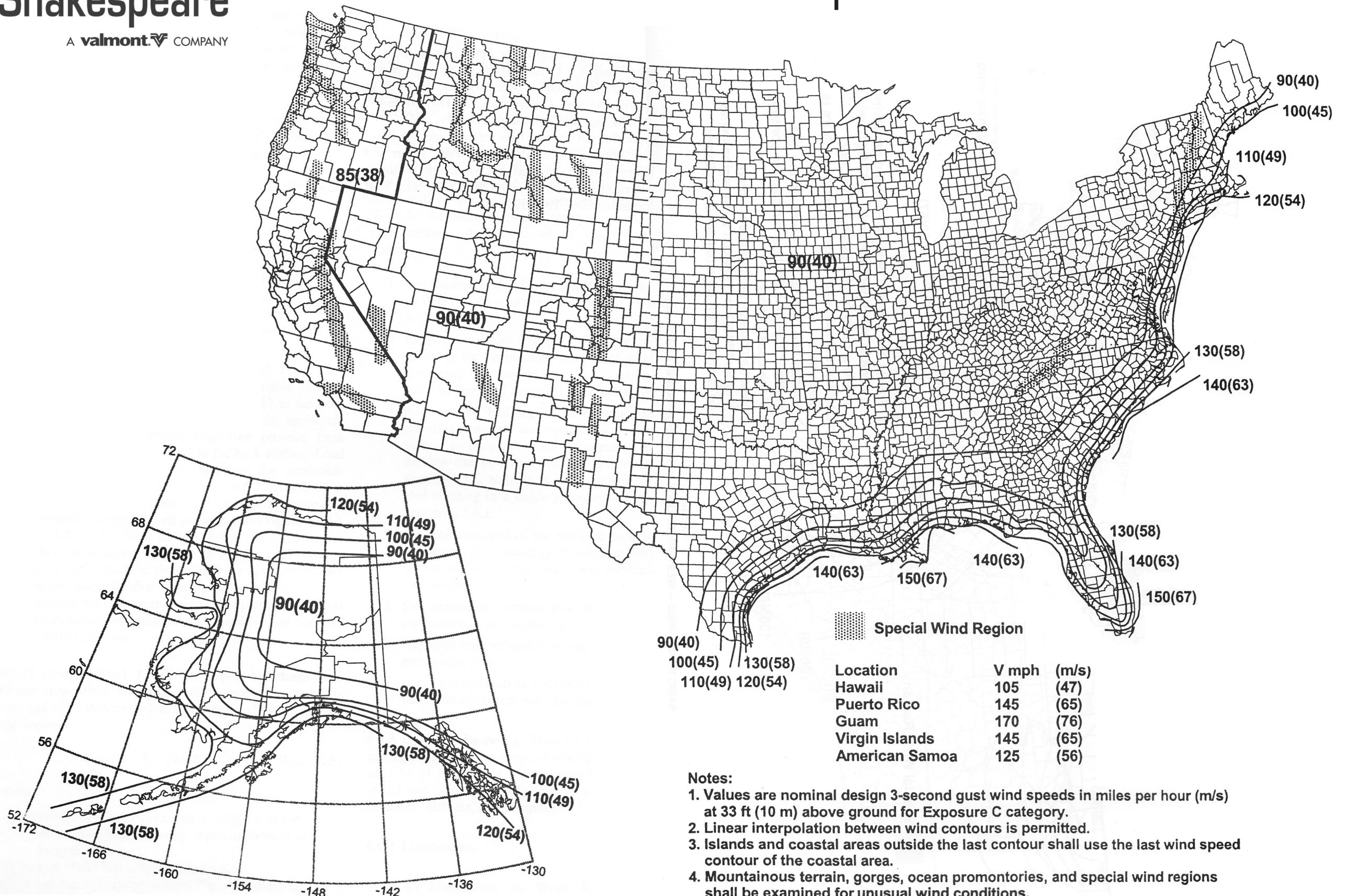
FIGURE 6-1 BASIC WIND SPEED
